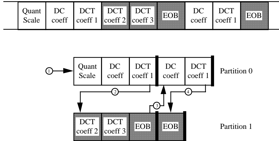
Figure 7-17 A segment from a bitstream with two partitions, with priority_breakpoint set to 64 (one (run, level) pair). The two partitions are shown, with arrows indicating how the decoder needs to switch between partitions.
